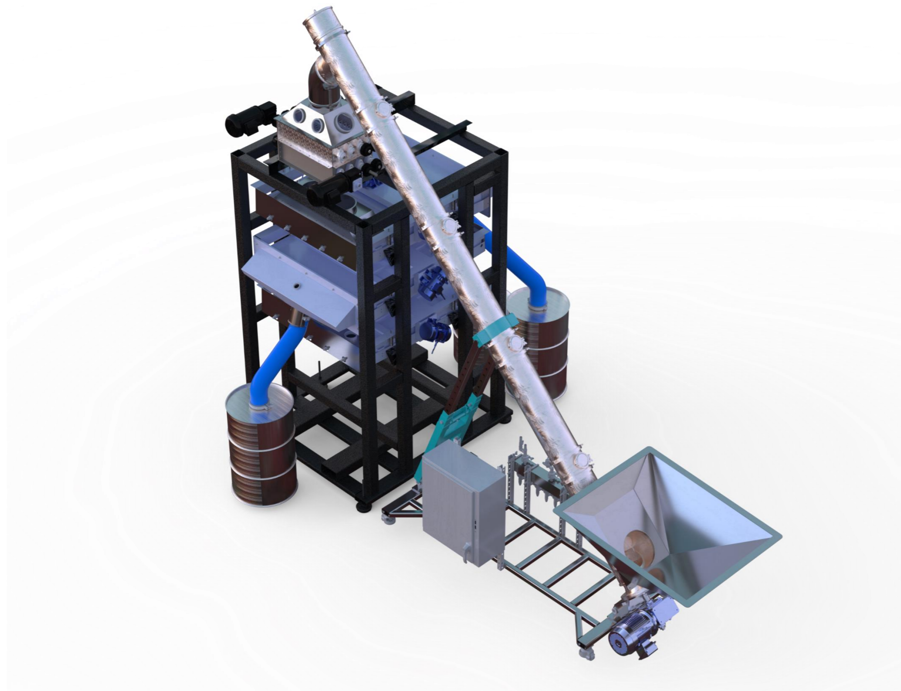
CryoSift Separator™ Production Model
