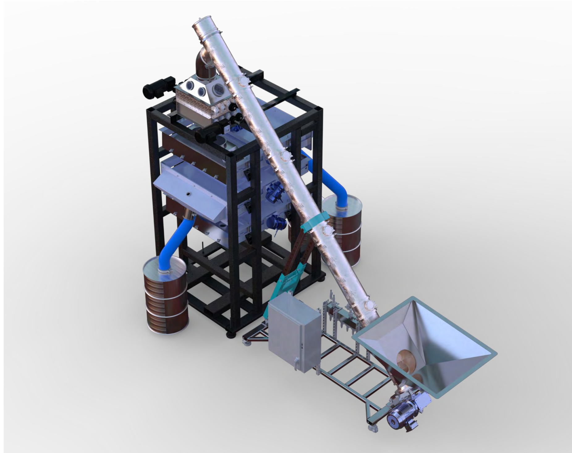
One-Skid CryoSift Separator™ Production Model
