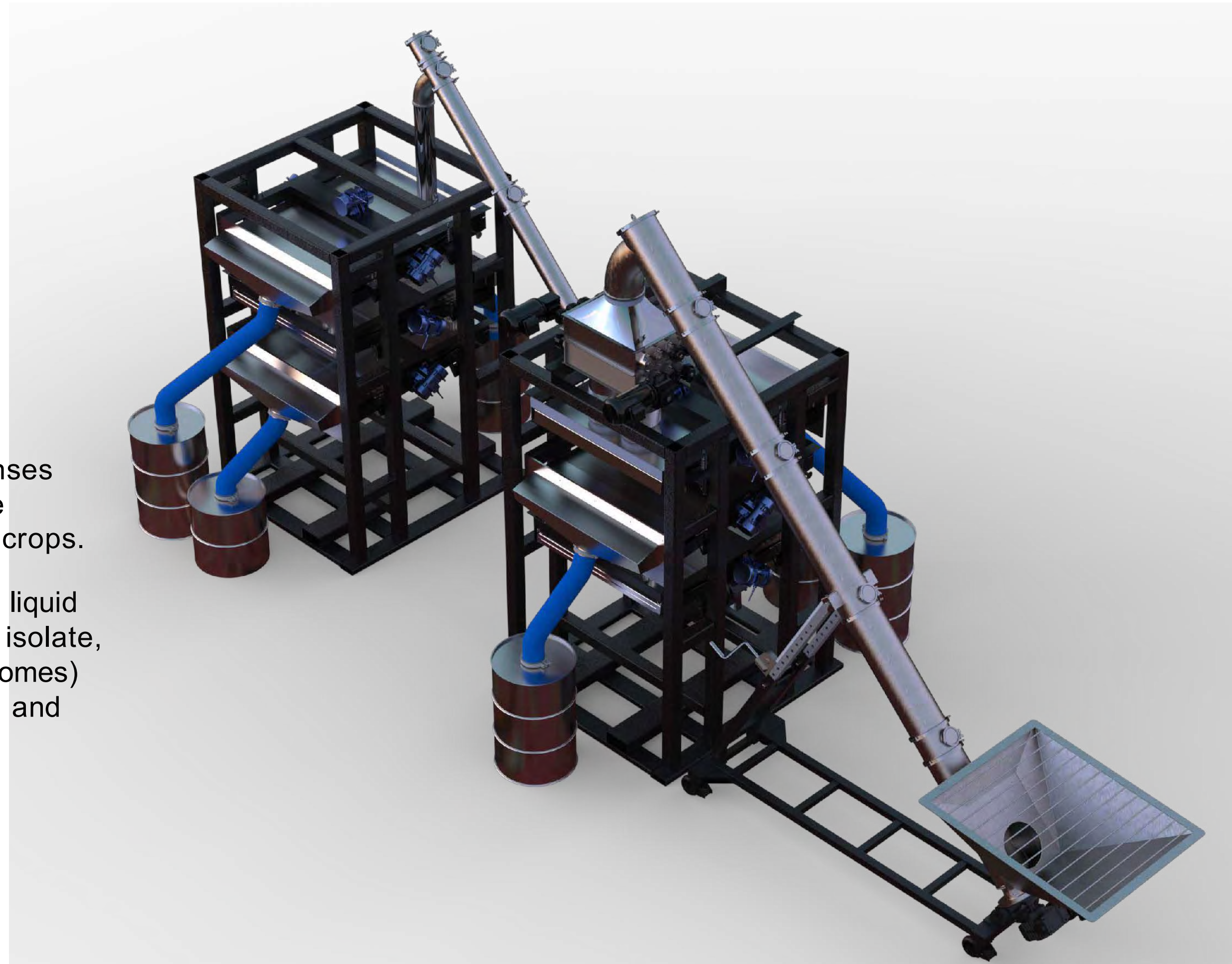
Two-Skids CryoSift Separator™ Production Model
